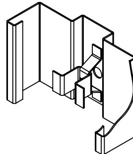
Compressions Anchor For slip on drywall frames
