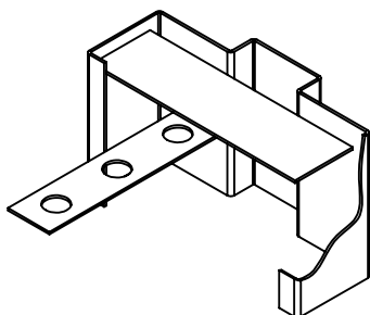
Loose T-Strap (Masonry)
