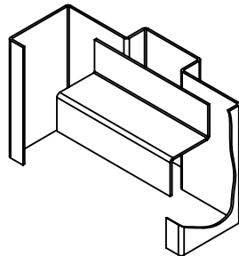
Recessed Z Anchor
