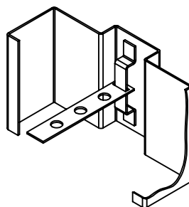
Welded T-Strap (Masonry)
